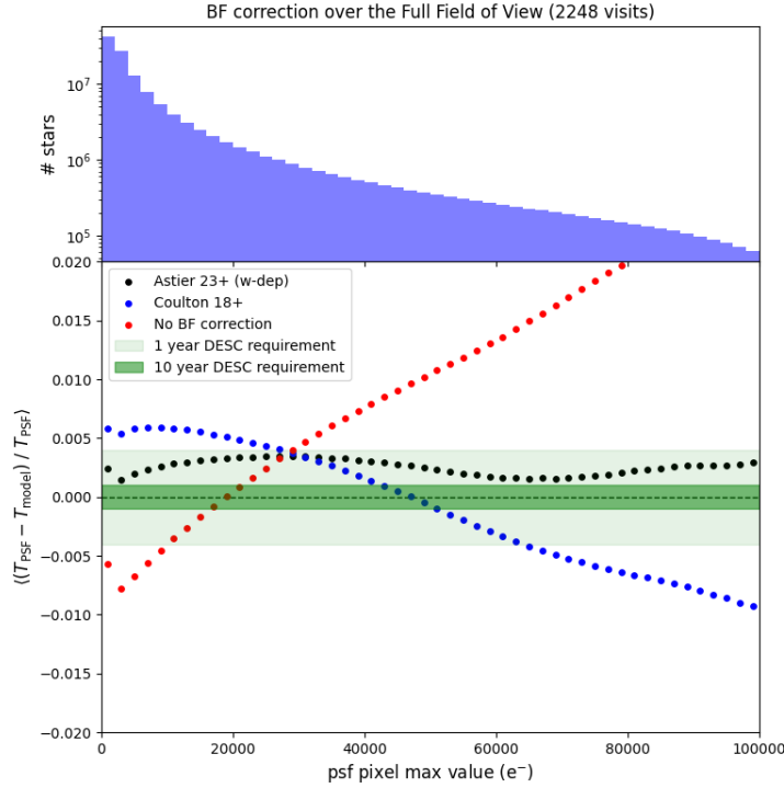
FIGURE 10: Brighter-fatter correction performance. The red curve shows the uncorrected flux-dependent PSF size residuals, the blue curve the current pipeline correction, and the black curve the new electrostatic model. The latter achieves sub-0.5% accuracy and removes the over-correction seen previously.
