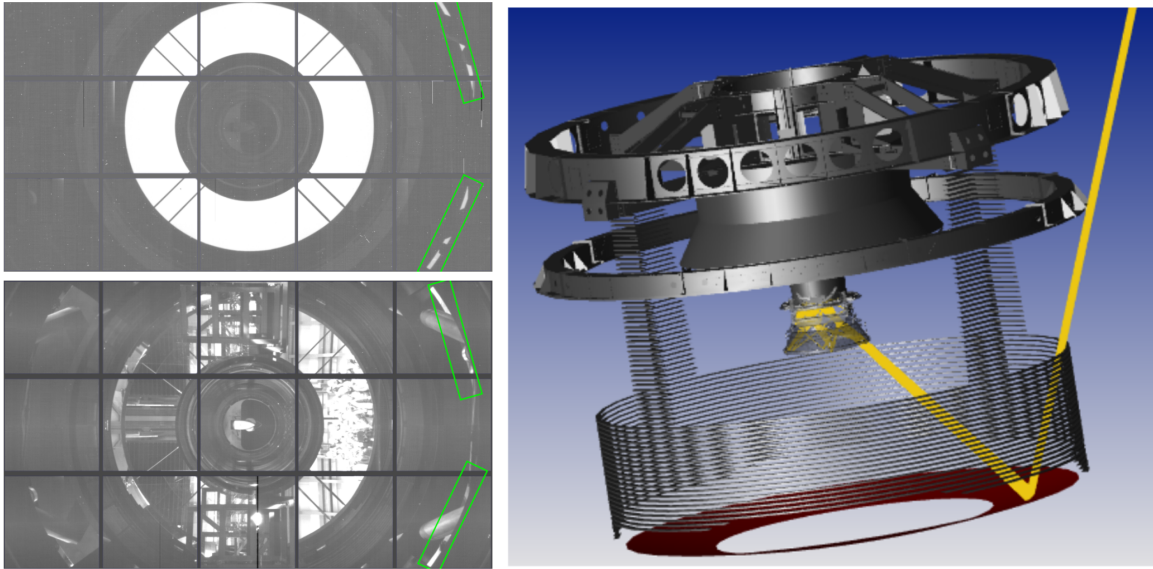
FIGURE 12: Identification of the light path responsible for the “Scratched Tape” artifact. Left : pinhole images taken on-sky during twilight (top) and in-dome (bottom). The unbaffled light path between the TMA mid-level and center-section baffles is identified with green boxes. Right : modeling in confirmed the existence of a direct off-axis light path through this gap, off of M1, and into the camera. Figure adapted from Drlica-Wagner et al. (SITCOMTN-166).
