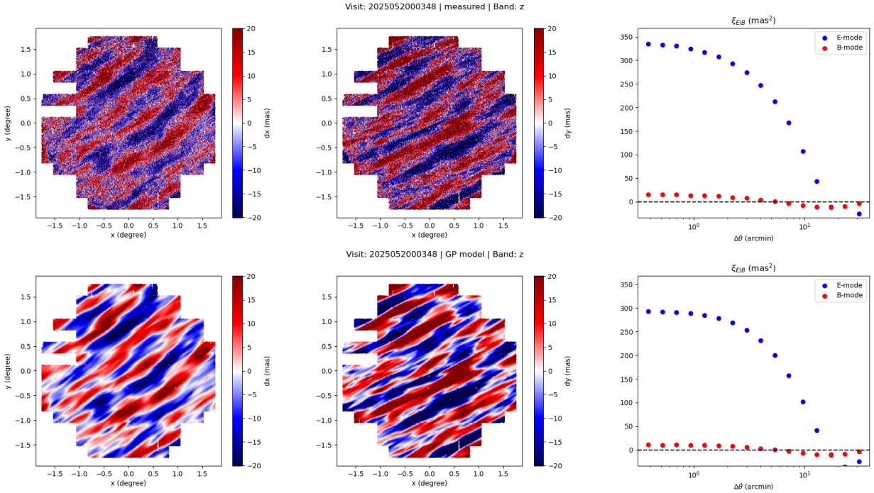
FIGURE 15: Gaussian-process modeling of atmospheric turbulence. The model captures large-scale correlated patterns in the residuals and reduces single-visit astrometric scatter by about 90%.
