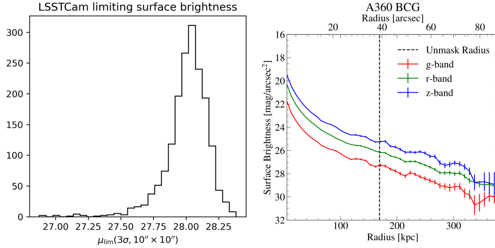
FIGURE 5: Low surface brightness performance. Left : Random sampling of g -band LSSTCam visits yields a limiting surface brightness of \sim 28 mag arcsec -2 . Right : LSSTCam Radial photometry around the BCG in Abell 360 confirms consistent surface brightness sensitivity across filters.
