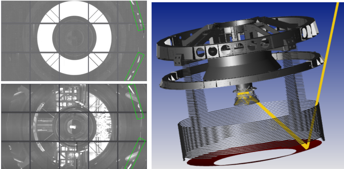
FIGURE 11: Identification of the light path responsible for the “Scratched Tape” artifact. Left: pinhole images taken on-sky during twilight (top) and in-dome (bottom). The unbaffled light path between the TMA mid-level and center-section baffles is identified with green boxes. Right: modeling in confirmed the existence of a direct off-axis light path through this gap, off of M1, and into the camera. Figure adapted from Drlica-Wagner et al. (SITCOMTN-166).
