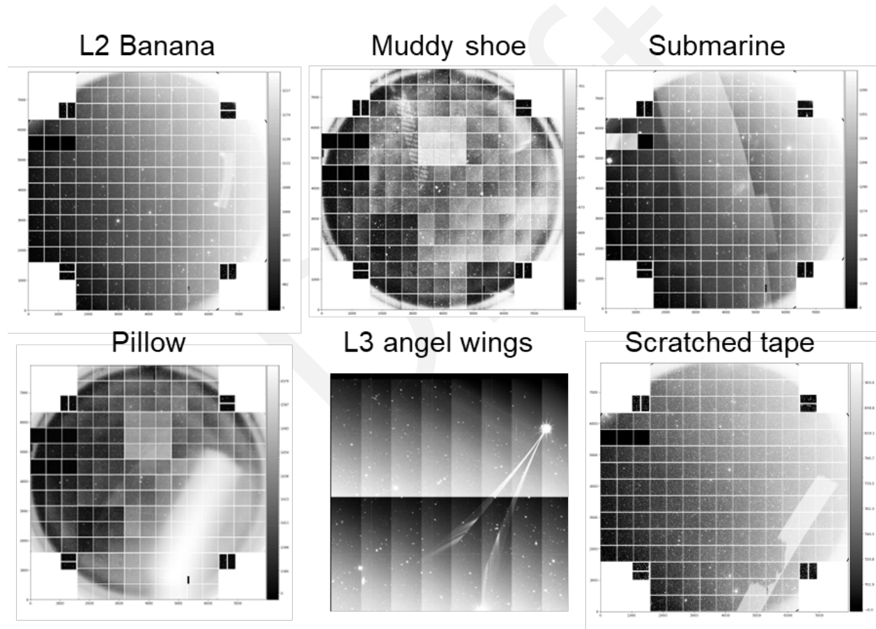
FIGURE 10: Examples of stray and scattered light features observed during LSSTCam commissioning. More than a dozen artifacts have been cataloged. Several of the most prominent artifacts have been traced to specific opto-mechanical origins. The incidence of stray and scattered light artifacts are expected to be significantly mitigated by the Light Wind Screen and additional baffling improvements.
