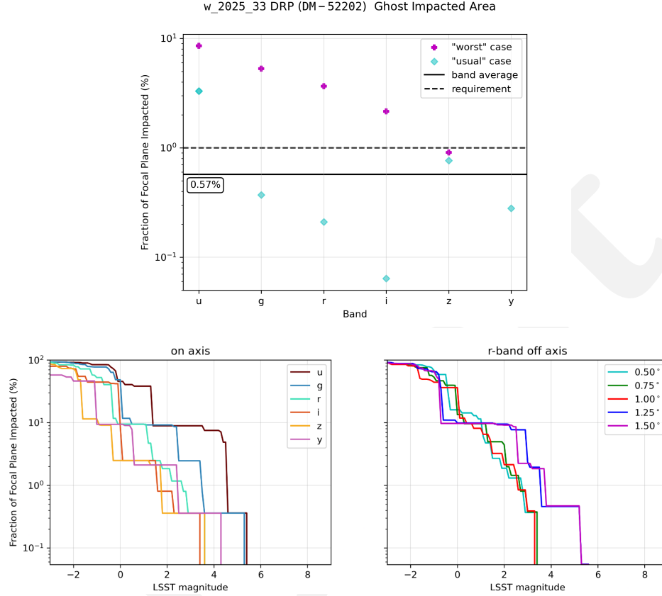
FIGURE 6: (Top) Fraction of the focal plane impacted by optical ghosts simulated with Batoid as a function of bandpass. The "usual case" impacted area was calculated using DRP visits while the "worst case" impacted area was calculated using visits that contained high amounts of ghosting selected by visual inspection. The mean loss is \sim 0.6\% across all filters, with worst performance in u and best in r and i , satisfying the requirement that ghost area loss remain below 1%. (Bottom Left) Impacted area as a function of simulated star magnitude in each band. (Bottom Right) Impacted area as a function of field position of the simulated star in r -band. The impacted area does not vary heavily with field position.
